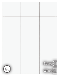
R20 Vertical groove spacing 200 mm Note: The following front widths have special groove spacings: 30 cm = 148 mm 45+90 cm = 223 mm 50 cm = 248 mm
